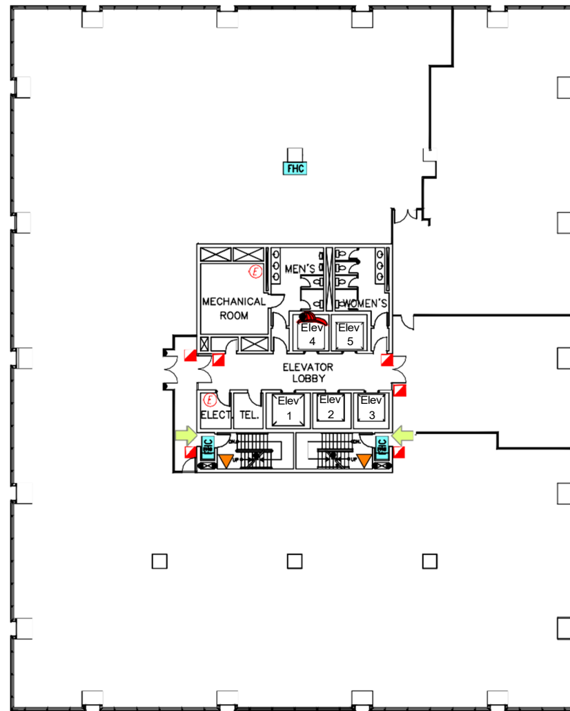
6th FLOOR
