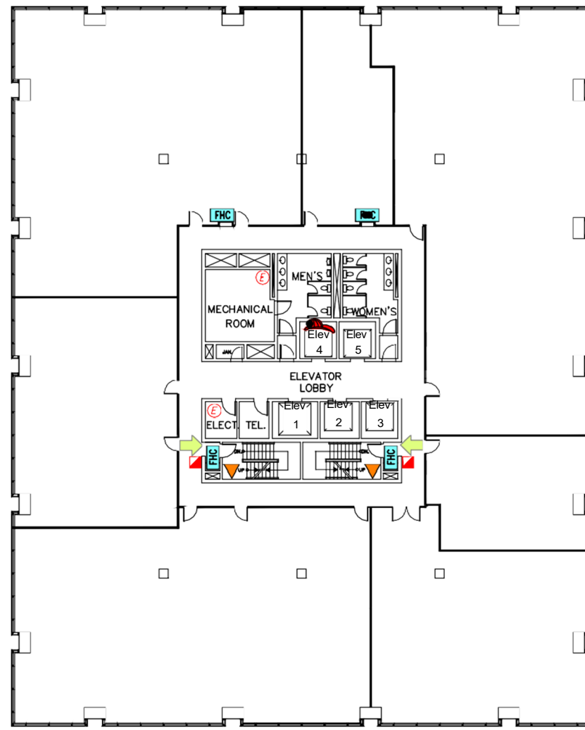
2nd FLOOR
