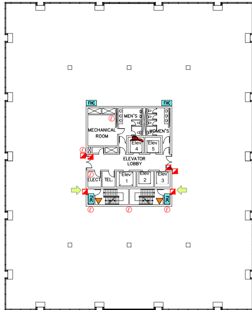
11th FLOOR
